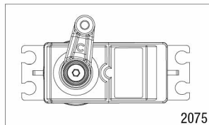
Servo Horn Position
