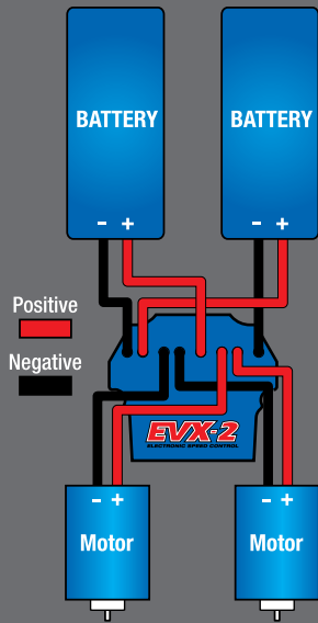
EVX-2 Wiring Diagram
