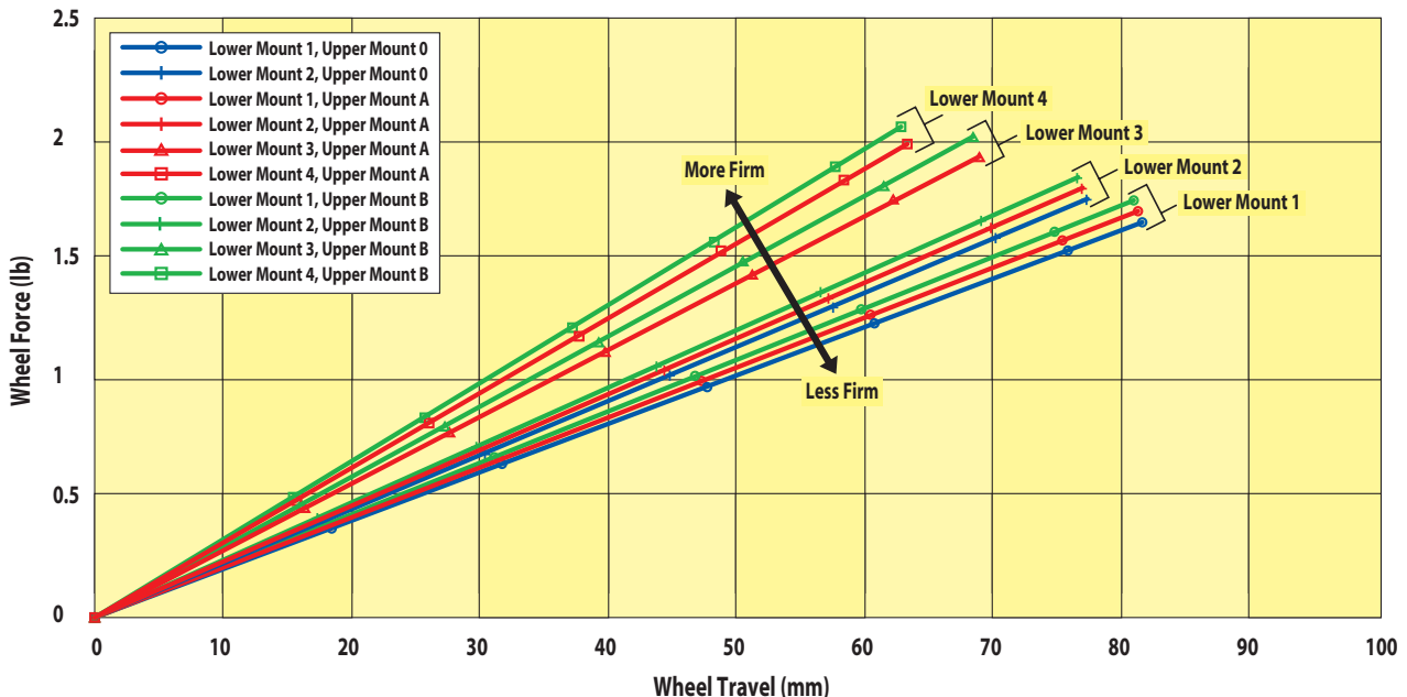
Wheel Force vs. Wheel Travel
